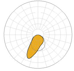
DA5525: Asymmetric 55° at 25° Tilt
