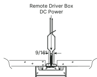
T1 - 9/16" Flat T-Bar Mount
