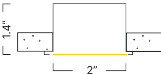
Flush Lens
