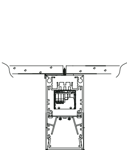
SC1 - Surface Mount Clip
