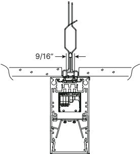
T2 - 9/16" Bolt Slot T-Bar Mount
