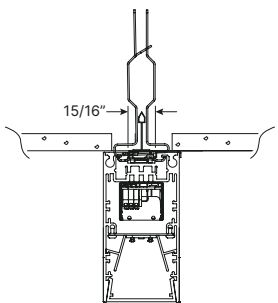
T3 - 15/16" Flat T-Bar Mount
