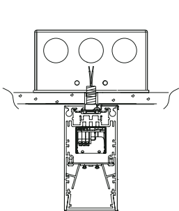
DJ - Drywall/J-Box Mount
