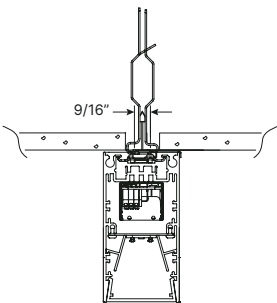
T1 - 9/16" Flat T-Bar Mount
