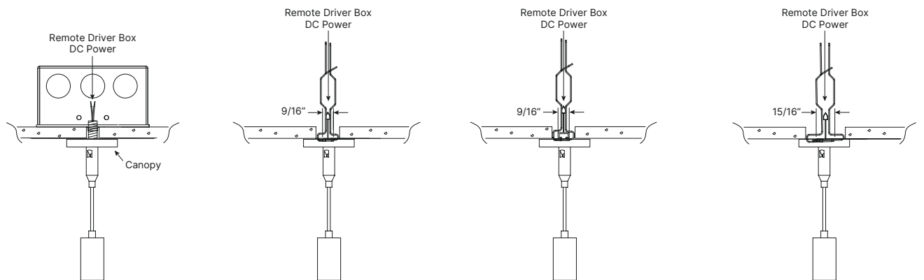
DJ - Drywall/J-Box Mount
