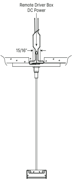
T3 - 15/16" Flat T-Bar Mount
