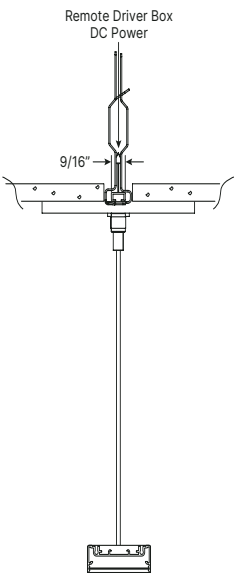
T2 - 9/16" Bolt Slot T-Bar Mount
