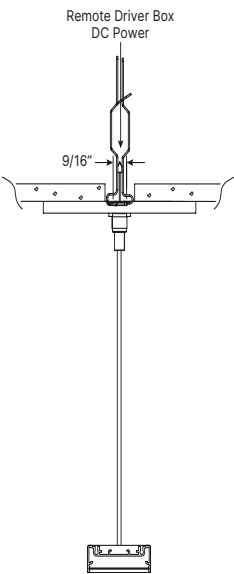
T1 - 9/16" Flat T-Bar Mount
